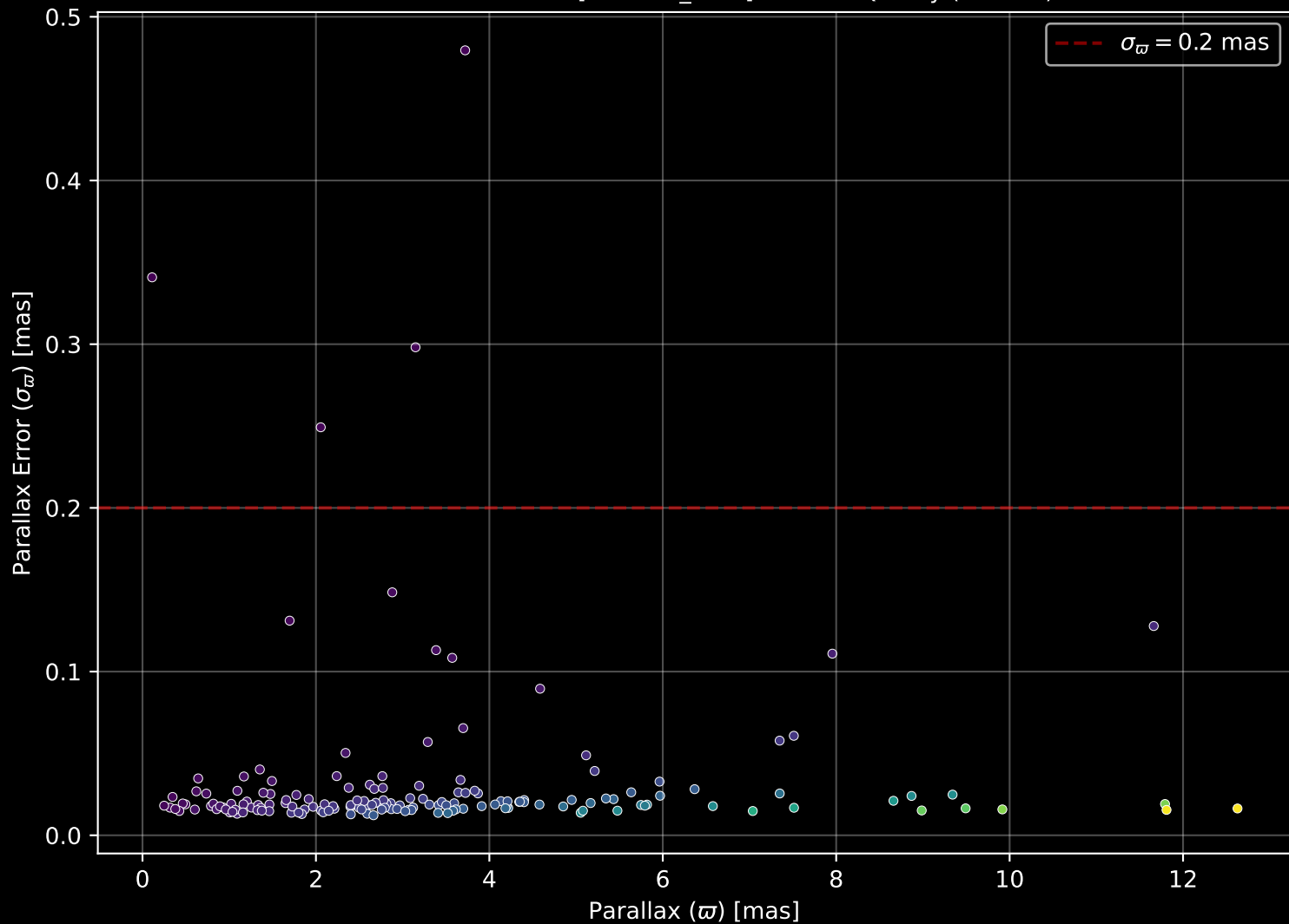
APOGEE DR17 Field: [198+36_MGA] Parallax Quality (n= 162)
