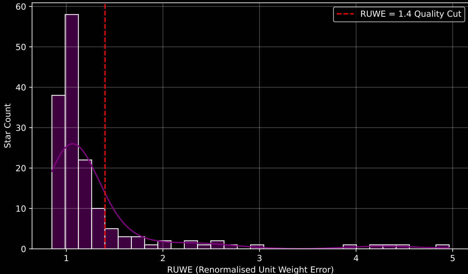
GAPOGEE DR17 Field [198+36_MGA] RUWE Distribution (n= 154)
