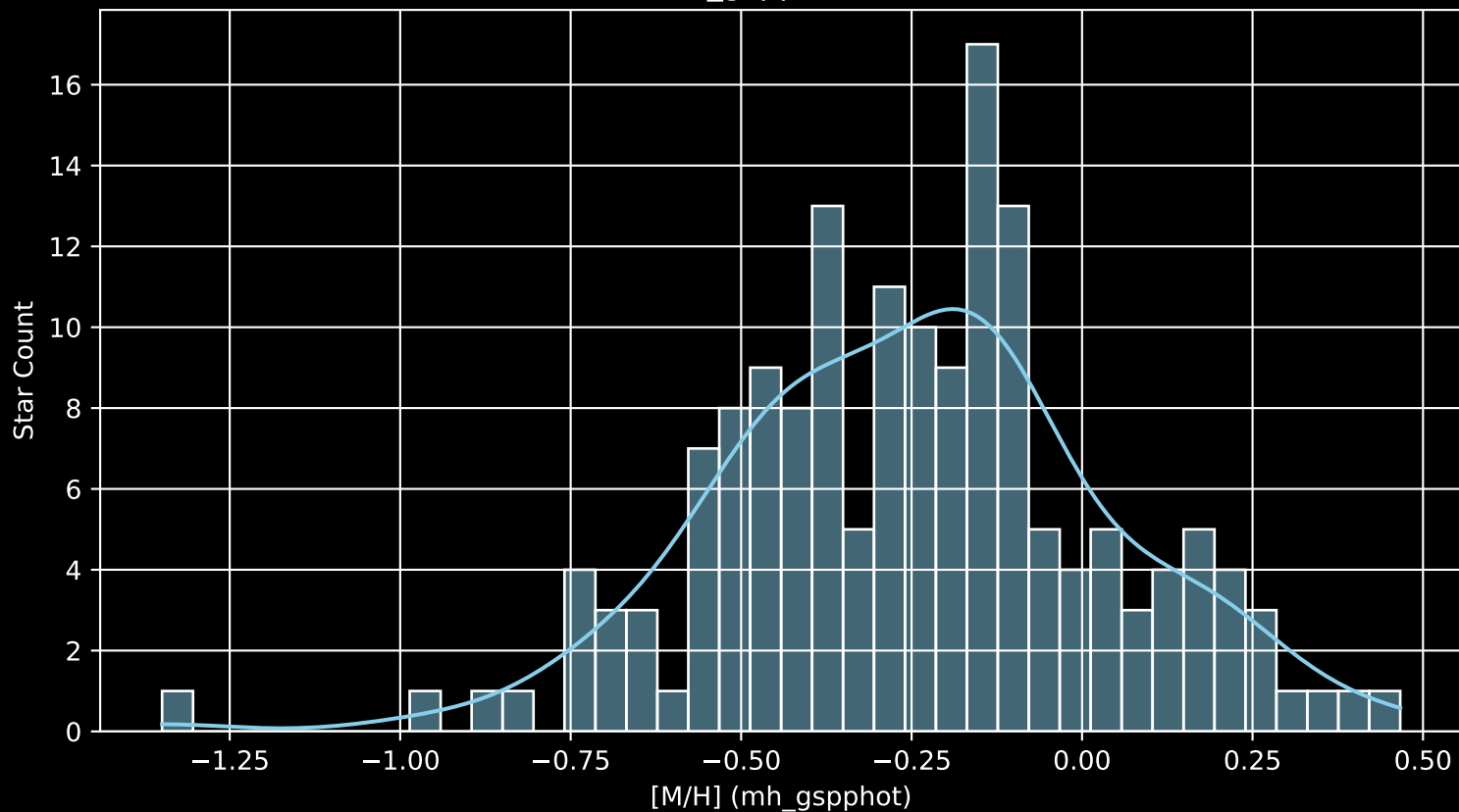
APOGEE DR17 Field: [198+36_MGA [M/H] (mh_gspphot) (n= 162)
