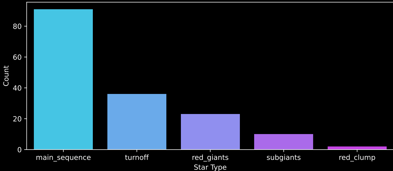
APOGEE DR17 Field: [198+36_MGA] Count plot of Star Type
