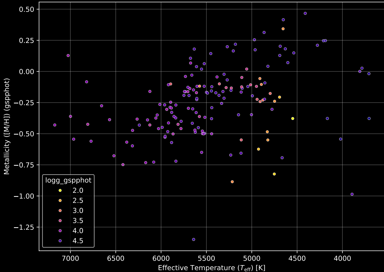
APOGEE DR17 Field: [198+36_MGA] Stellar Population Parameters (n= 162)
