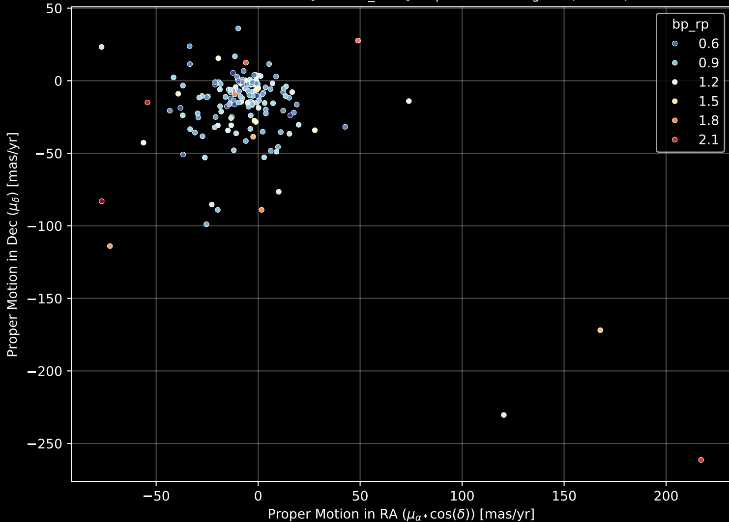
APOGEE DR17 Field: [198+36_MGA] Proper Motion Diagram (n= 162)
